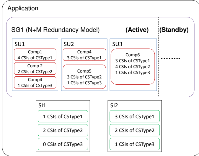
Figure 3. The active part of an example of SG with N+M redundancy model
