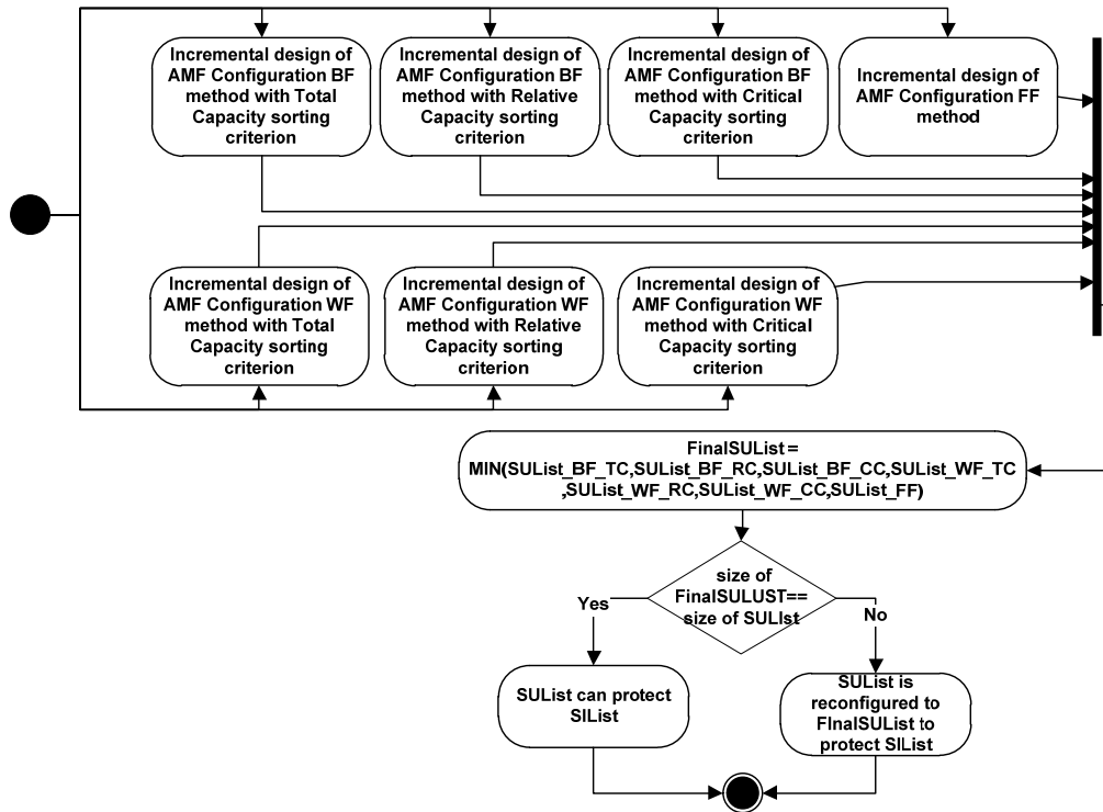
Figure 6. Overview of the incremental design approach
