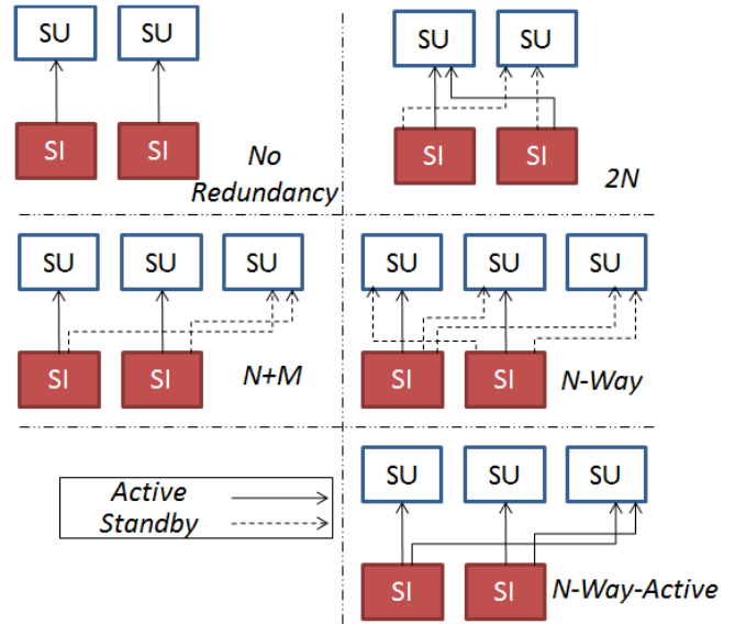
Figure 1. Redundancy models defined in the AMF specification
