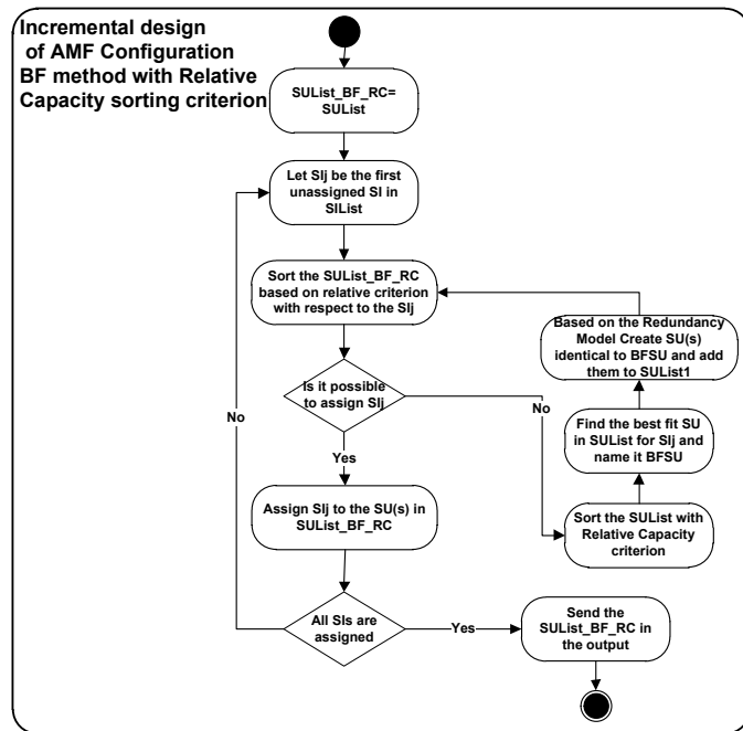
Figure 4. Incremental AMF configuration design using BF method with relative capacity sorting criterion
